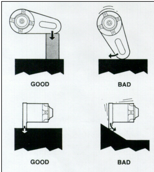
Figure 4 Reaction Plate must not slip when torque is applied
