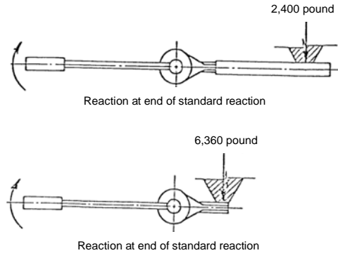
Figure 1 Reaction forces increase the closer the reaction point is to the multiplier.
