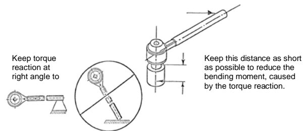
Figure 2 Minimize bending moments created by the torque multiplier's reaction.
