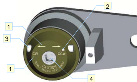
Fig 1. Input End Detail
