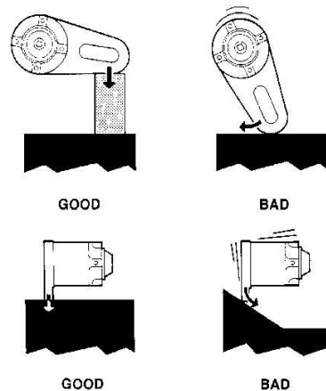
Figure 3 Keep reaction anchor perpendicular to the reaction point.
