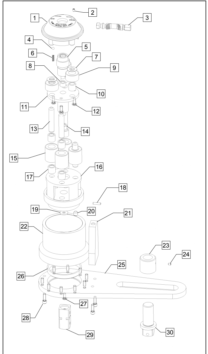
Figure 5 Torque Multiplier – Parts List Exploded View
