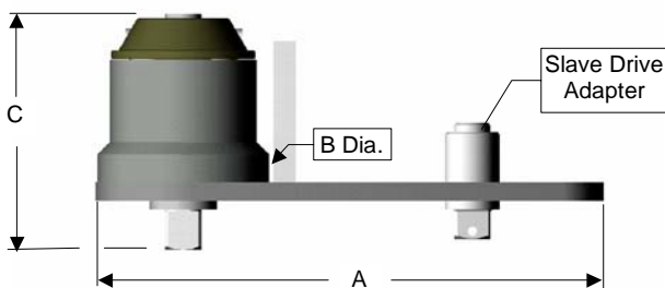
Fig. 3 Overall Torque Multiplier Dimensions
