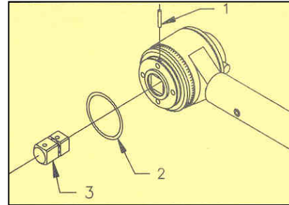
Figure 1. Replacing Output Square Drive Assembly
