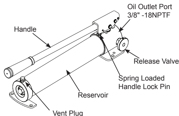
Figure 2 - Model 5HS2S100 Components
