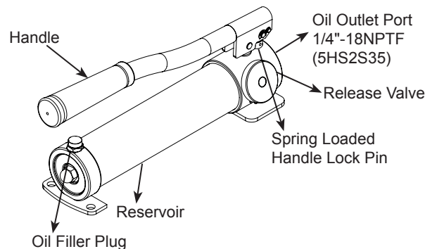
Figure 1 - Model 5HS2S35 Components
